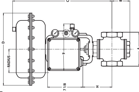
2-WAY or 3-WAY w/ DL84 or 84XR & 760 Positioner
