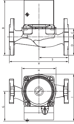
Wilo-Star S, Drawing no.: 5
