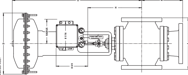
3-WAY w/ DL115 or 115XR & 760 Positioner
