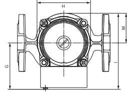
Wilo-Star, Drawing no.: 1
