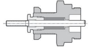
Adjustable Graphite Packing
