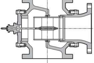
2932 Three-Way Diverting/Mixing Valve
