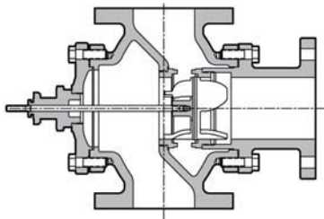
2930 Three-Way Mixing Valve
