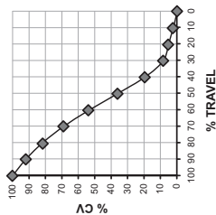
2-WAY VALVE TYPICAL FLOW CURVE
