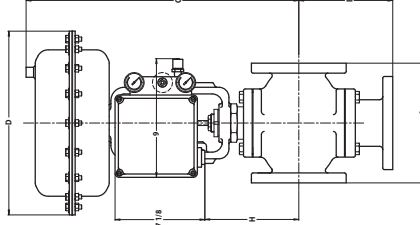
3-WAY w/ DL84 or 84XR & 760 Positioner
