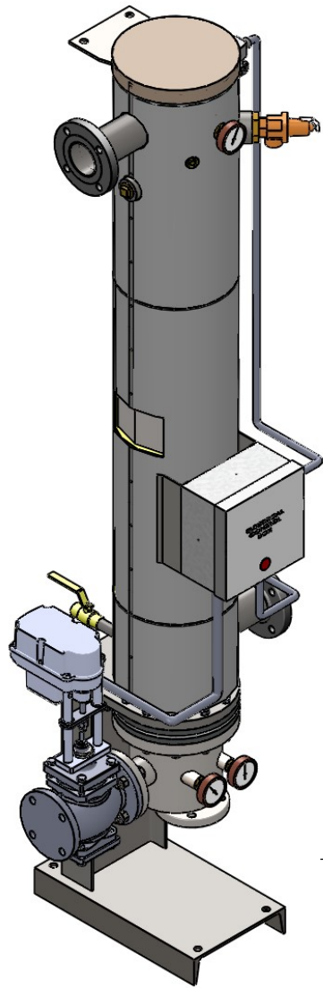
ISOMETRIC VIEW
