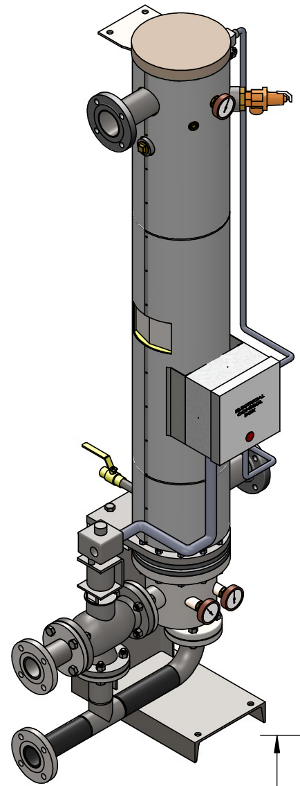
ISOMETRIC VIEW
